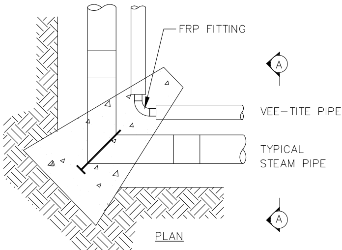
CONDENSATE SERVICE
