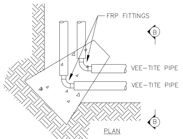
HOT/CHILLED WATER SERVICE
