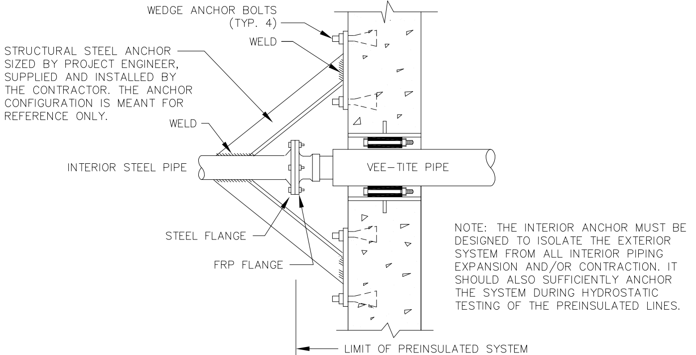
TYPICAL ANCHOR AT WALL PENETRATIONS NO SCALE
