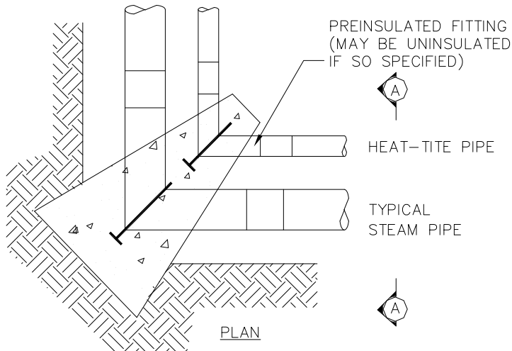
CONDENSATE SERVICE
