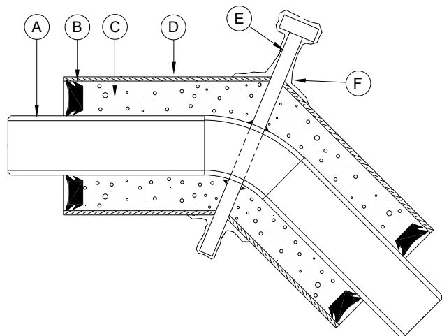
45° ELBOW WITH ANCHOR NO SCALE
